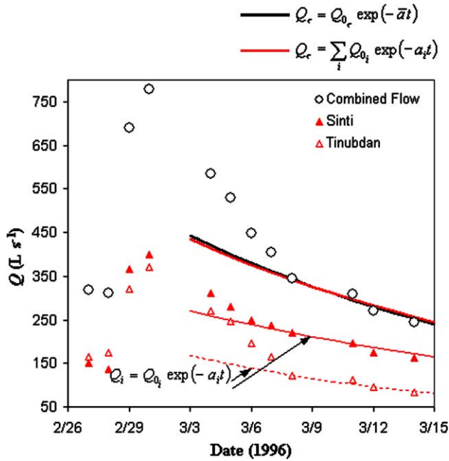
Fig. 6. Hydrographs for the two large springs, Sinti and Tinubdan (red in web version), and the combined flow from all of the springs (black). The exponential recession curves from Eq. (8) are superimposed on the data. The linear reservoir constants, a_i , are taken from Table 2 and \bar{a} is the average of the a_i coefficients from the two large springs.
